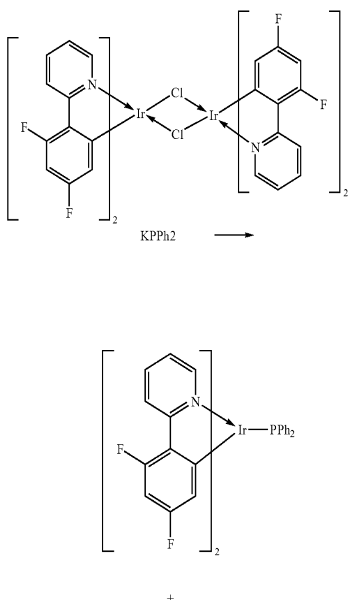
Reaction scheme I
