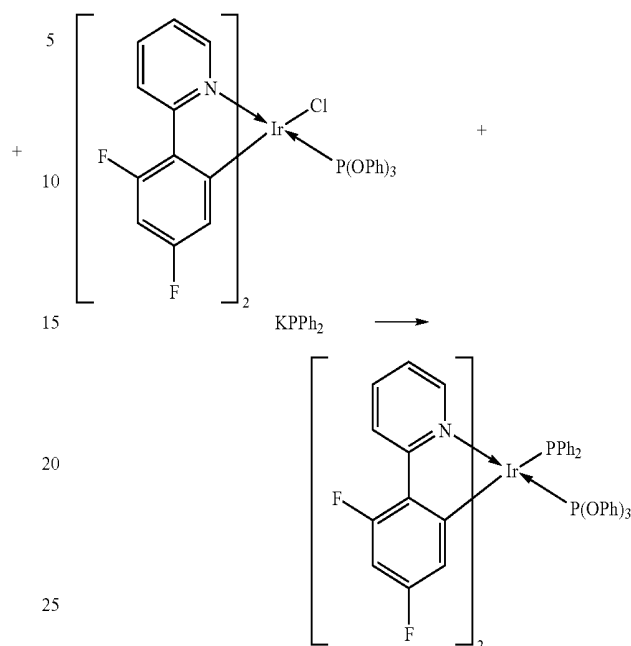
Reaction scheme II
